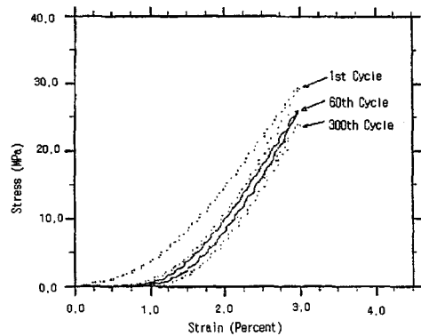
Fig. 3 Stress-Strain responses with cycles for an A-type test
