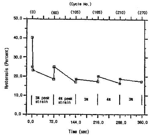
Fig. 8 Average hysteresis (%) in the C-type tests
